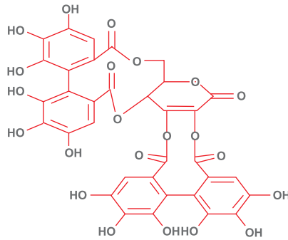
Emblicanin B
