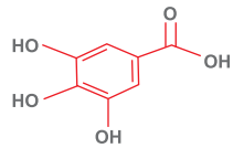
Gallic Acid
