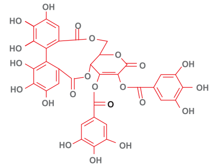
Emblicanin A
