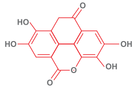
Ellagic Acid
